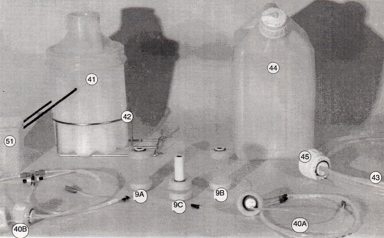
Figure E-9. ABI 433A reagent bottles, tubing, and reaction vessels.
