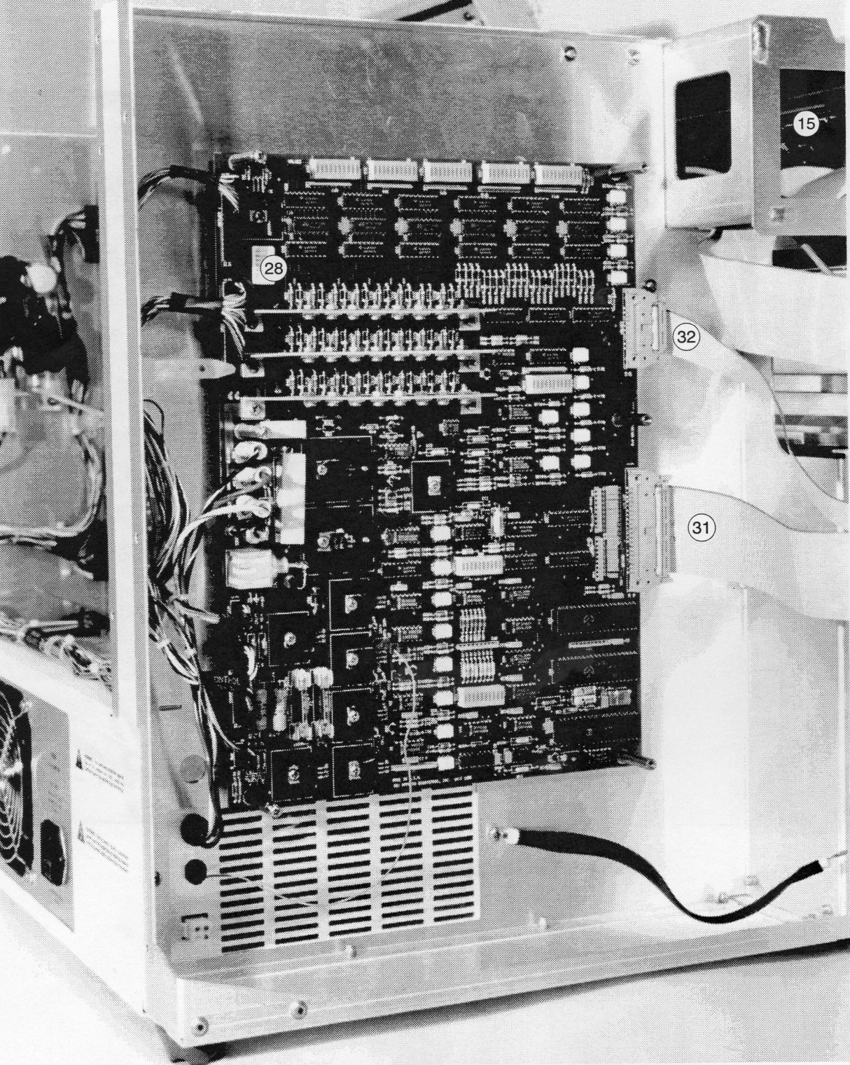
Figure 5-4. Left side of the APL 432A with the panel detached
