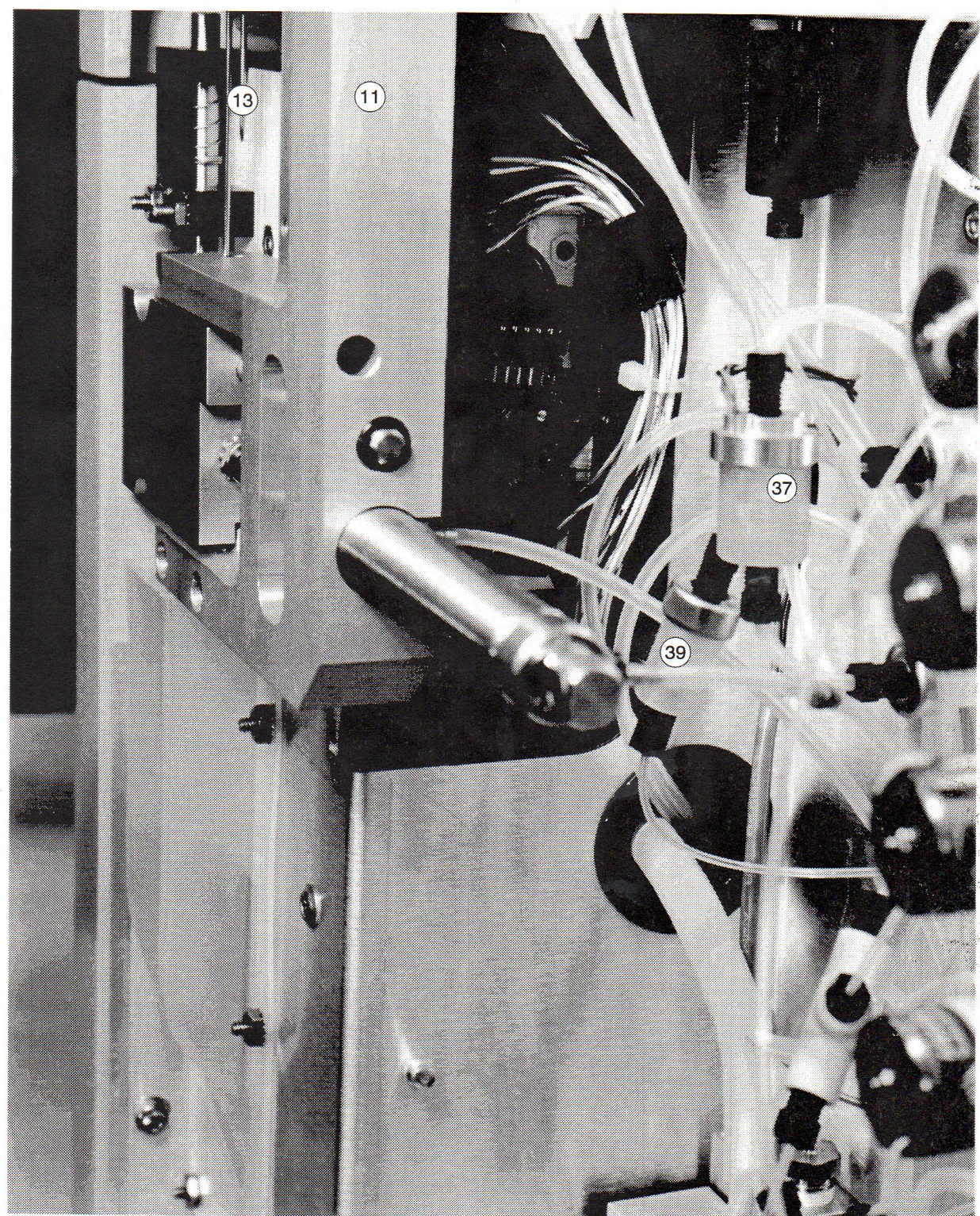
Figure F-6. Conductivity flow cell close up
